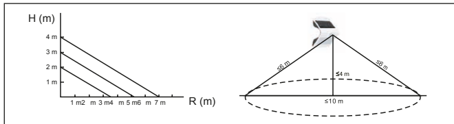
Fig.8: Installation - Portée
